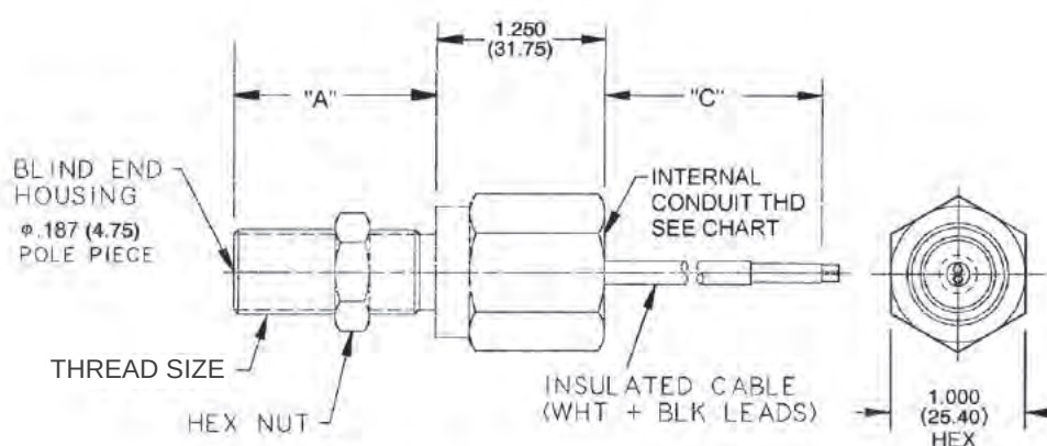
Figure 1: Dimension Drawing
